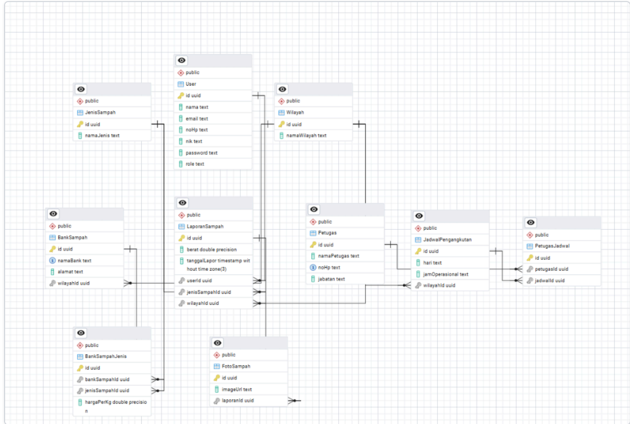
Gambar 8. Diagram Lengkap Entity Relationship Diagram (ERD) PostgreSQL di pgAdmin
